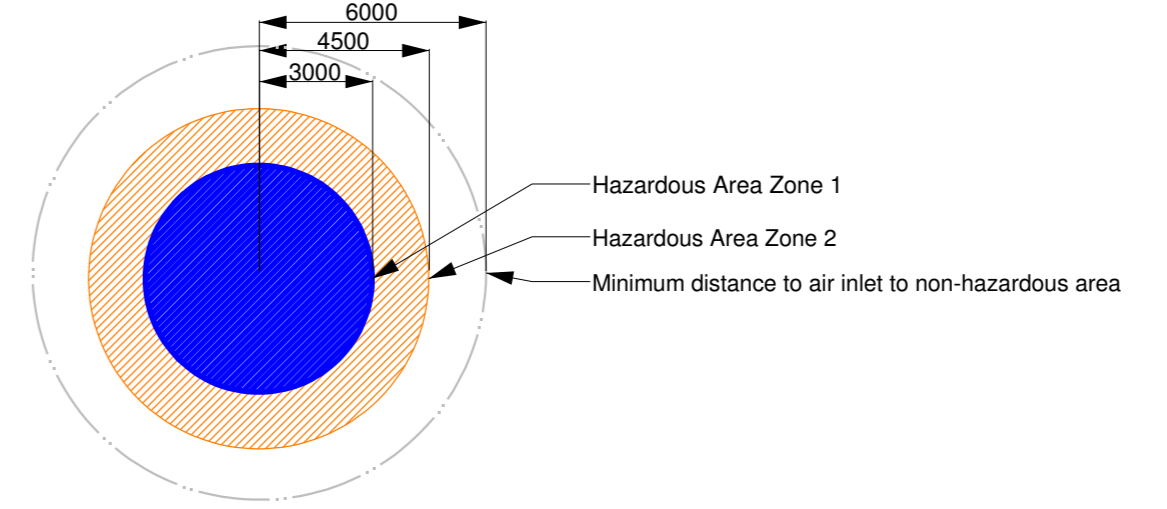
Ventilation Outlet Hazardous Area Zone 1
