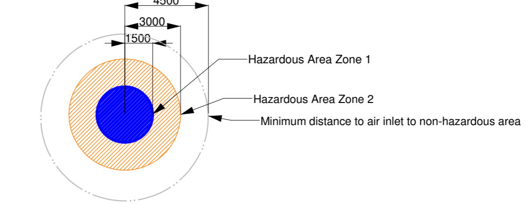
Ventilation Outlet Hazardous Area Zone 1
