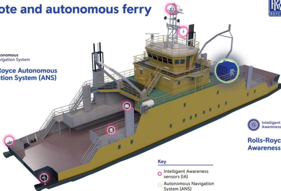
Figure 2: Falco - perhaps the first autonomous full scale ferry
