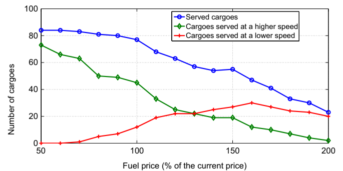
Fig. 2. The number of served cargoes, the number of cargoes served at a higher-than-preferred speed and the number of cargoes served at a lower-than-preferred speed for different fuel prices.
