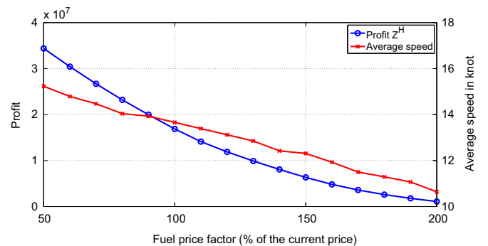
Fig. 3. The profit and average speed in knots for different fuel prices.
