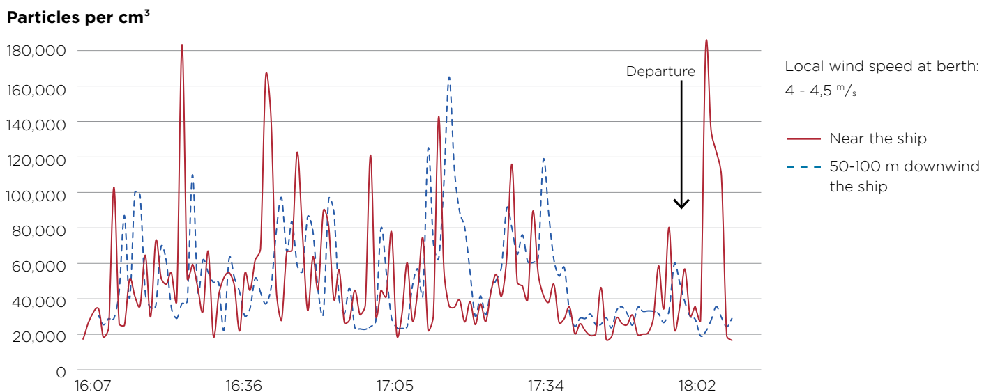
Figure 3: Air pollution with ultrafine particles from cruise ships at Oceankaj in Port of Copenhagen.
