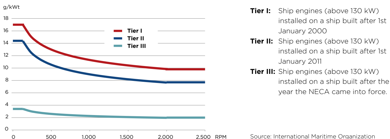
Figure 5: Regulation of NO x from shipping
